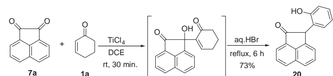
Scheme 2. Synthesis of 2-(2-hydroxyphenyl)-2H-acenaphthylen-1-one ( 20 ) from 1,2-acenaphthenequinone ( 7a ) and cyclohex-2-enone ( 1a ).
