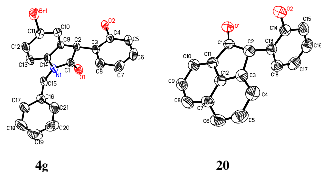
Figure 2. ORTEP diagrams of 4g and 20 (Hydrogen atoms are omitted for clarity).
