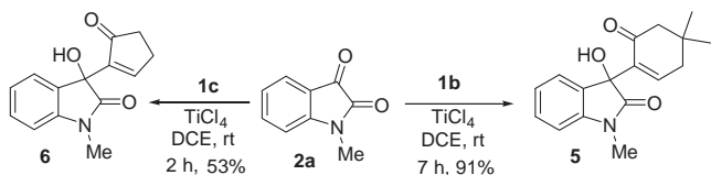
Scheme 1. Synthesis of Baylis–Hillman alcohols ( 5 , 6 ) from 1-methylisatin ( 2a ) and cyclic enones ( 1b , c ) in the presence of \text{TiCl}_4 .
