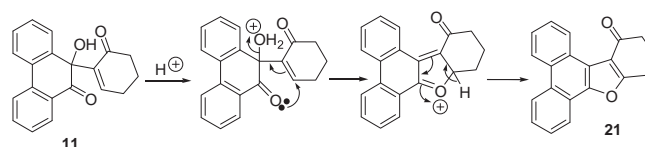
Scheme 3. Plausible mechanism for synthesis of furan derivatives.
